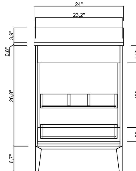
BACK VIEW
